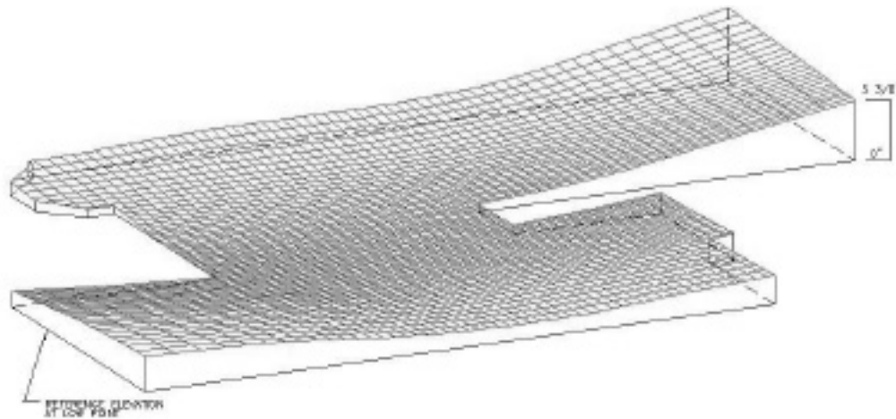
Figure 1. Three Dimensional Representation of Total Out-of-Levelness Floor Plan A (28 Total Beam Tendons)
