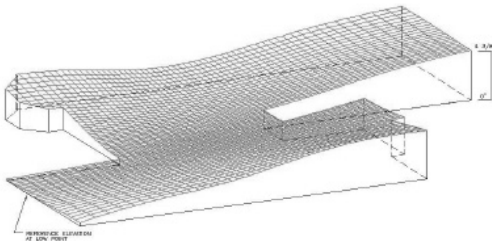
Figure 2. Three Dimensional Representation of Total Out-of-Levelness Floor Plan A (23 Total Beam Tendons)
